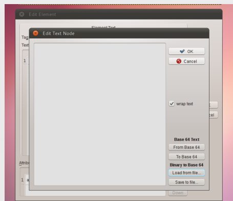
3 Insert a child text node and select "Load from file..."
